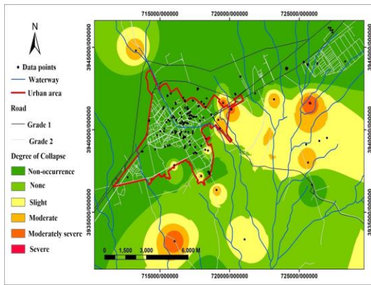
شکل ۱۱. Classification of Semnan and suburbs collapsible potential according to ASTM D5333
