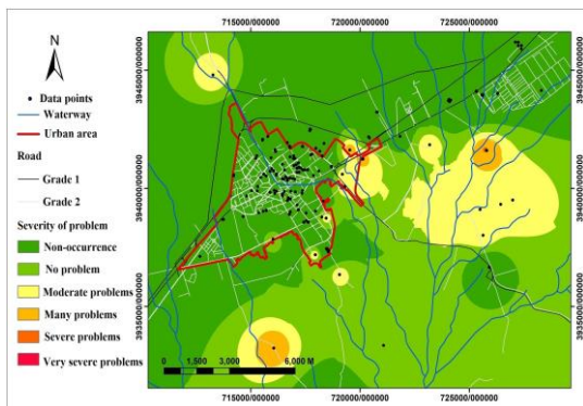
شکل ۱۱. Classification of Semnan and suburbs collapsible potential according to J. Jennings, K. Knight
