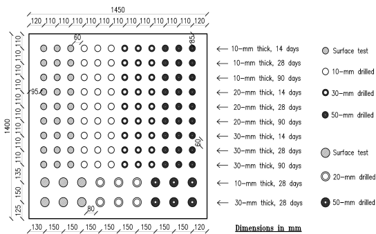
Fig. 4. Positions of pull-off tests for different discs and ages
