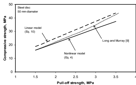
Fig. 7. Comparison of relationships between pull-off strength and compressive strength for steel disc
