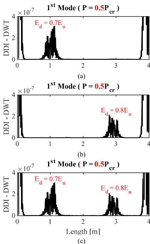
Fig. 7. DDI diagram of the 1 st mode resulting from discrete wavelet analysis of the db8 function for the (a) D1, (b) D2 and (c) D3 damage state
