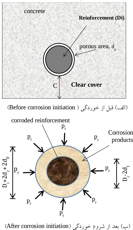
Fig. 3 The state of the space around the rebar and the stresses caused by the increased volume of the corroded material
