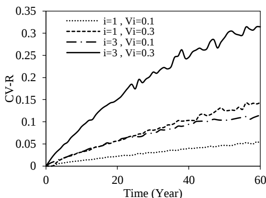
Fig. 17. The effect of probabilistic properties of corrosion current density on the coefficient of variation of the bond strength ratio
