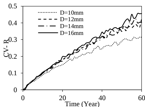
Fig. 14. The coefficient of variation of bond ratio for different bar diameter ( i_{cor} = 3 \mu A/cm^2 )
