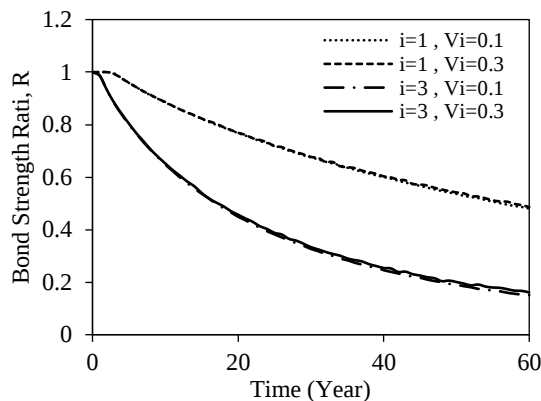
Fig. 16. The effect of probabilistic properties of corrosion current density on the average of the bond strength ratio
