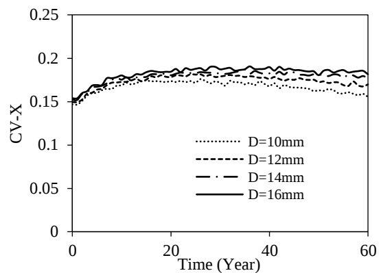
Fig. 12. The coefficient of variation of corrosion degree for different bar diameter ( i_{cor} = 3 \mu A/cm^2 )
