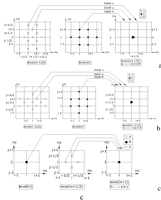
Fig. 2. a) Discretization U-momentum b) Discretization V-momentum c) Discretization of the continuity equation
