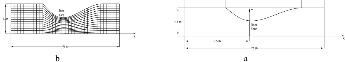
Fig.3.a) The studied area, the convergent – divergent experimental flume in the study of Bellos et al, 1992 b) a sample of meshing in the desired area
