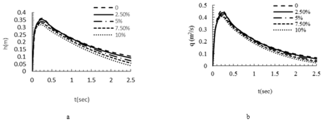
Fig. 7. Comparison of discharge and water surface elevation in site of dam-break with and without wall side slope of dam
