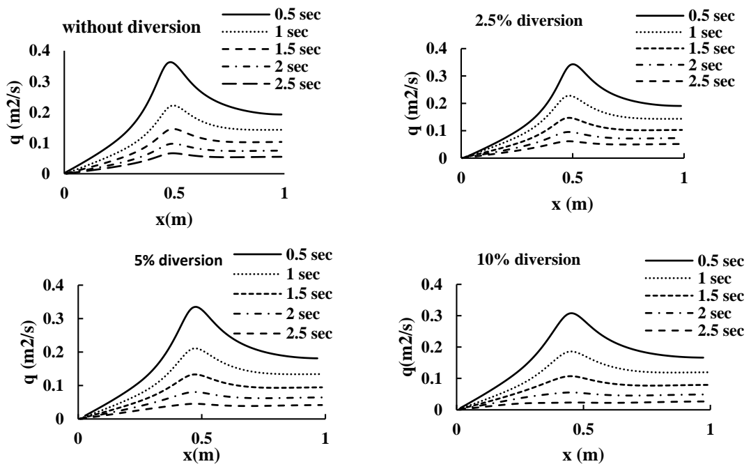
Fig. 8. Comparison of discharge on center line on dam break site with different side slope of wall da
