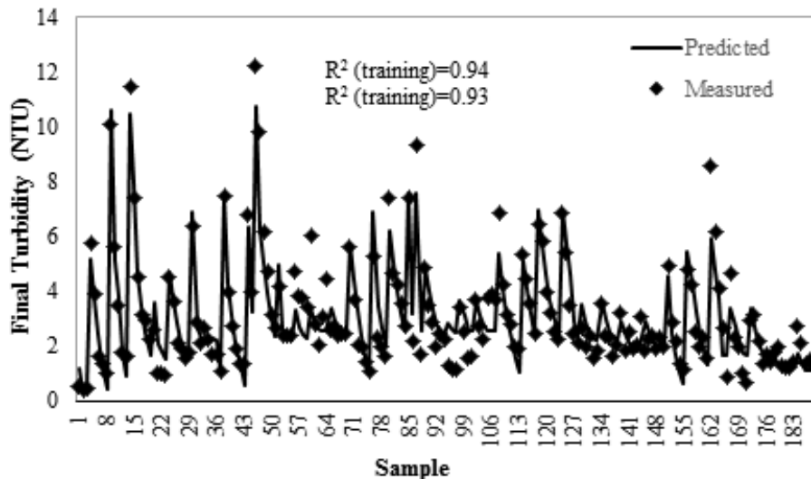
Fig. 7. The Predicted Final Turbidity by Fuzzy Regression model
