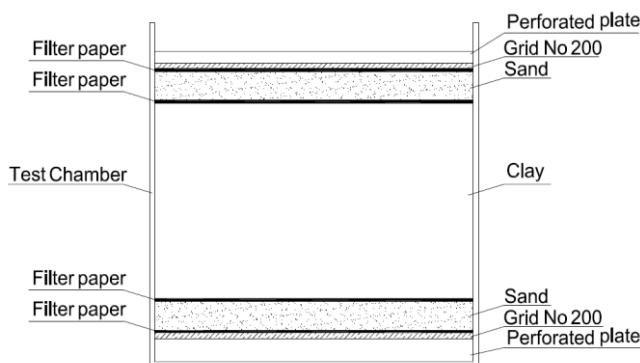
Fig. 5. Schematic diagram of the laboratory model test setup
