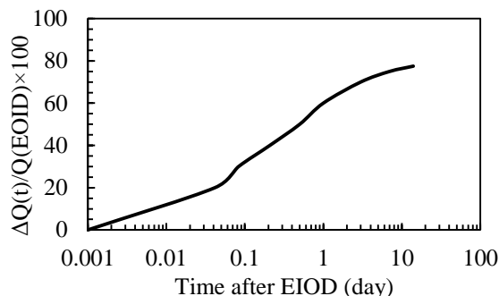
Fig. 9. Increase in pile capacity over time from pile static load tests at different times.
