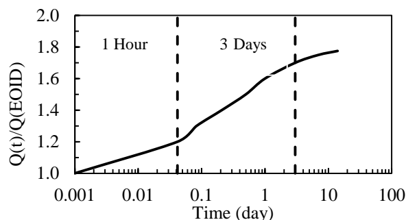
Fig. 10. Normalised Pile capacity versus time on log scale
