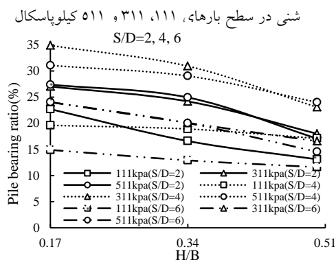
Fig. 9. Variations of the Pile bearing ratio with different thicknesses of cushion at 111, 311, and 511 kPa load levels
