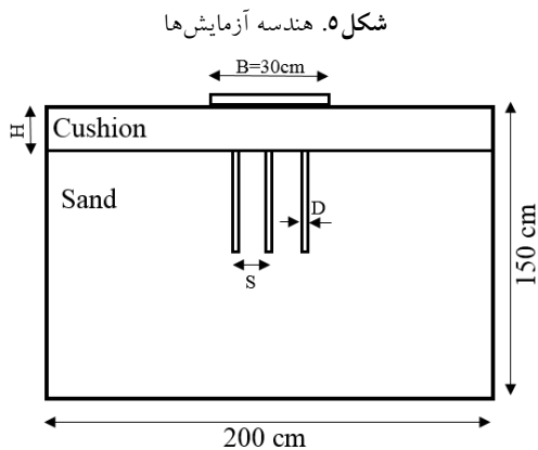
Fig. 5. Geometry of tests
