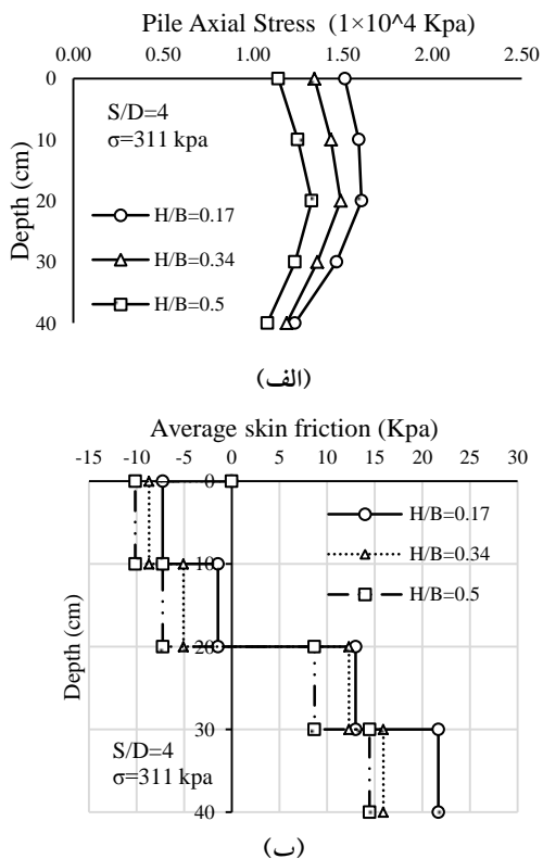
Fig. 11. Variations of axial stress and frictional stress along the corner pile (P3) in different thicknesses of the cushion
