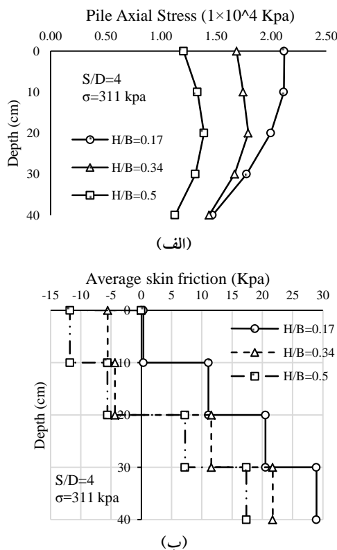
Fig. 10. Variations of axial stress and frictional stress along the central pile (P1) in different thicknesses of the cushion
