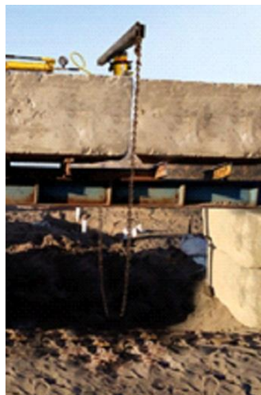
Fig. 3. Attachment of chain to the beam on the jack
