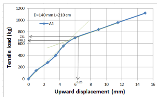
Fig.5. The application of tangent lines and 6.25-mm displacement methods
