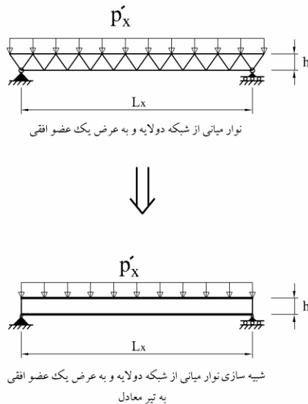
Fig. 2. Modeling of the double layer to estimate the deflection
