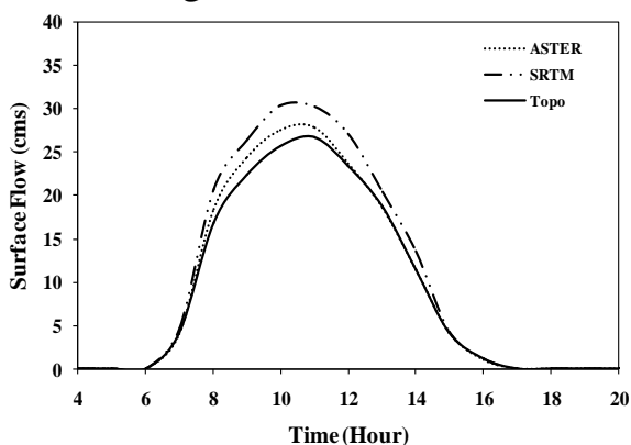
Fig. 17. Simulated hydrograph in different DEM sources (50m)
