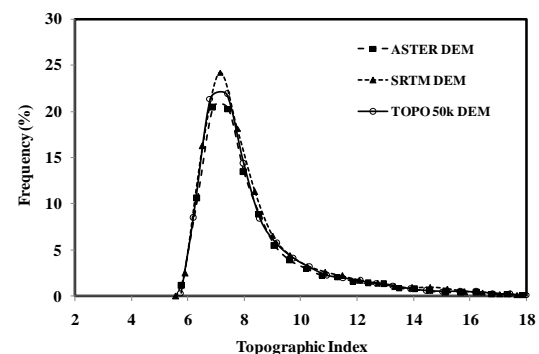
Fig. 7. Frequency distribution of TopoIndex (200m)
