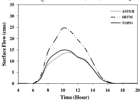
Fig. 16. Simulated hydrograph in different DEM sources (30m)
