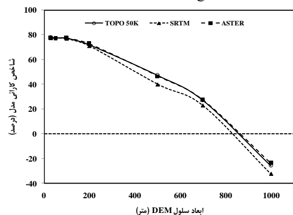
Fig. 15. The effect of DEM resolution on the performance of TOPMODEL (hourly flows)
