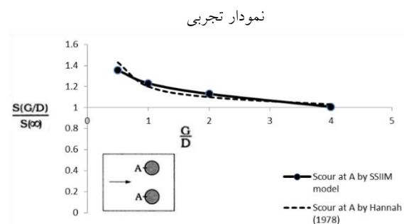
Fig 12. Comparison between scour level calculated by the model and measurements of Hannah (1978) at the front region of piers
