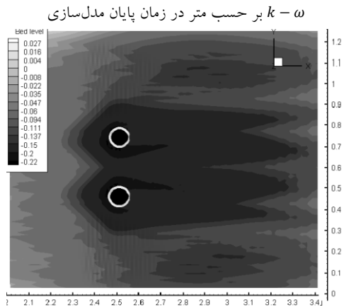
Fig 11. Contours of scour depth simulated using k - \omega turbulence model at the end of simulation
