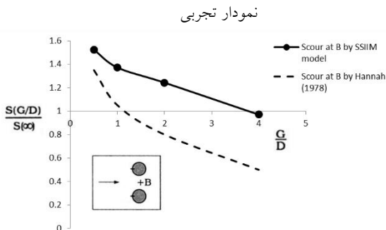
Fig 13. Comparison between scour level calculated by the model and measurements of Hannah (1978) at the mid-region of piers
