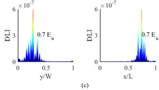
Fig. 7. 2 nd mode DLI diagram of the D2 damage state with the damage severity (a) 10%, (b) 20% and (c) 30%
