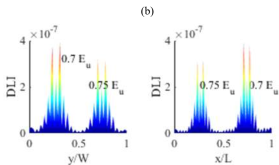
Fig. 9. 1 st mode DLI diagram of the D3 damage state with the damage severity (a) 10%, (b) 20% and (c) 30%
