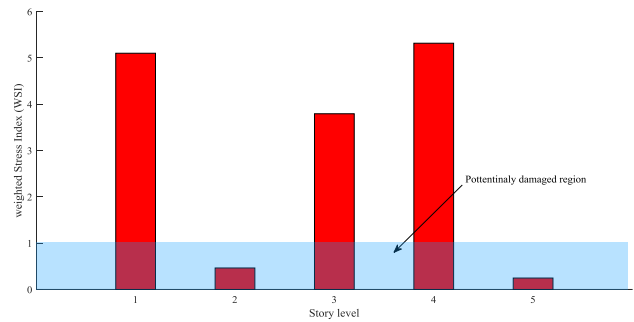
Fig. 18. WSI for each brace of steel frame floors for (5%, 20%)
