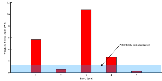
Fig. 24. WSI for each brace of steel frame floors for (10%, 20%)
