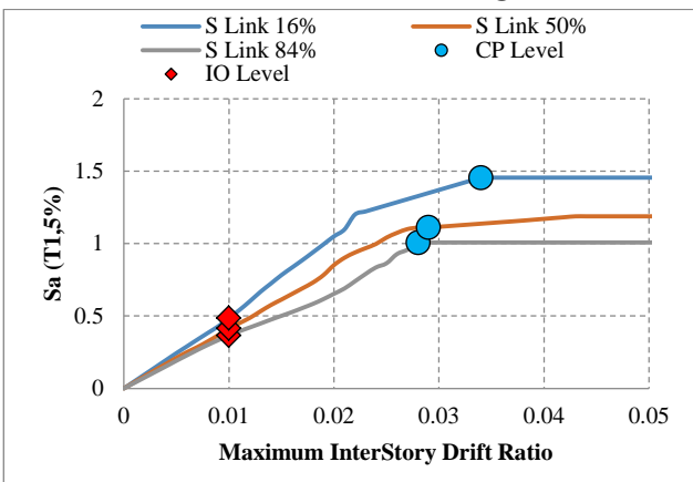
g) 15-story frame with shear link
