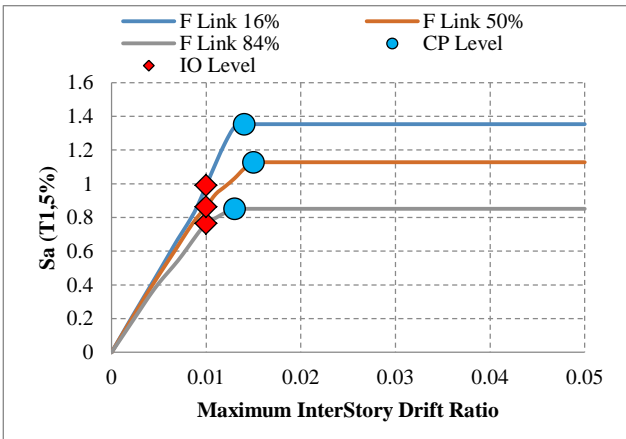
f) 10-story frame with flexural link
