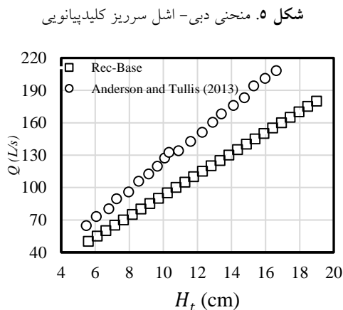
Fig. 5. Q versus H_t for piano key weir
