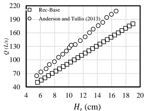
Fig. 5. Q versus H_t for piano key weir
