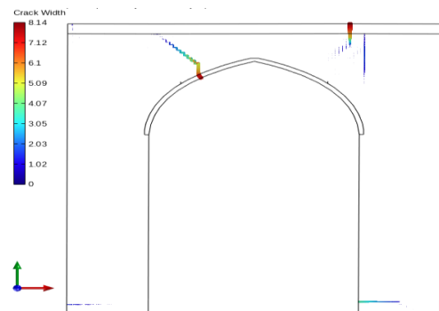
Fig. 19. The distribution pattern of cracks at the maximum shear capacity for the wall with 0.2 MPa pre-compression gravity load intensity (average displacement of 22.8 mm at the top of the wall)
