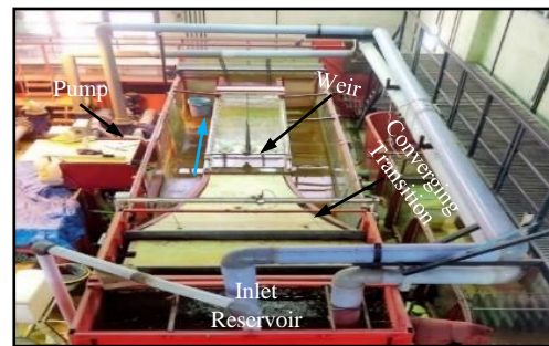
Fig. 3. Experimental flume
