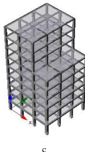
Fig. 4. Geometry properties of the 9-story structure a-plan configuration b-2-D-frame c-3-D-building
