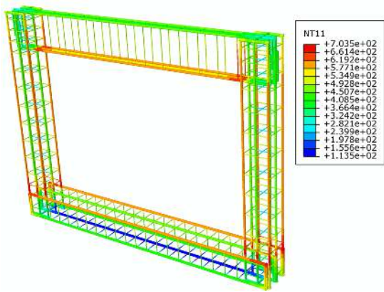
Fig. 11. Temperature distribution in steel reinforcements of SBFT frame
