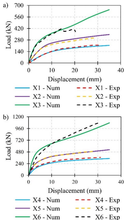
Fig. 5. Comparison numerical and experimental load-displacement curves.
