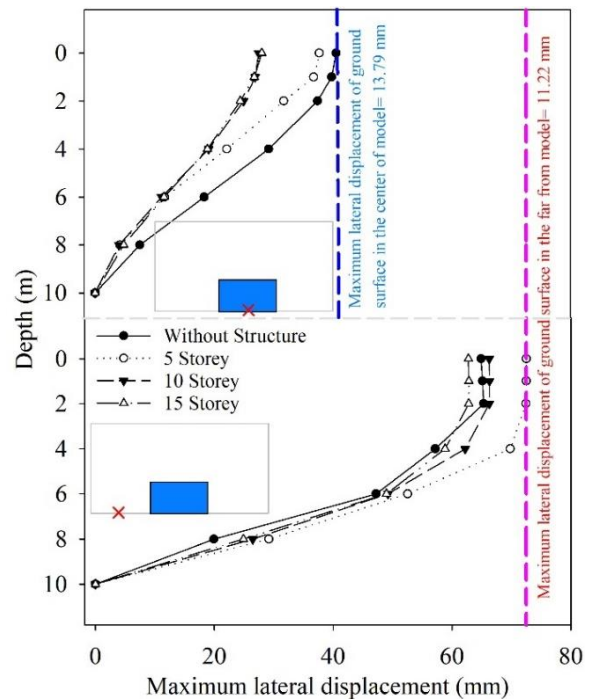
Fig. 7. Maximum lateral displacement of soil with 5 \times 5 DGCs in the center and far from the center of without and with 5-15-storey structures subjected to the 0.25g El-Centro earthquake
