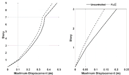
Fig. 15. Distribution of maximum floor displacement, El Centro, PGA=0.5g
