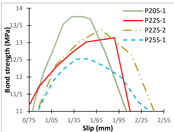
Fig. 11. Bond strength - slip diagram in maximum stress range
