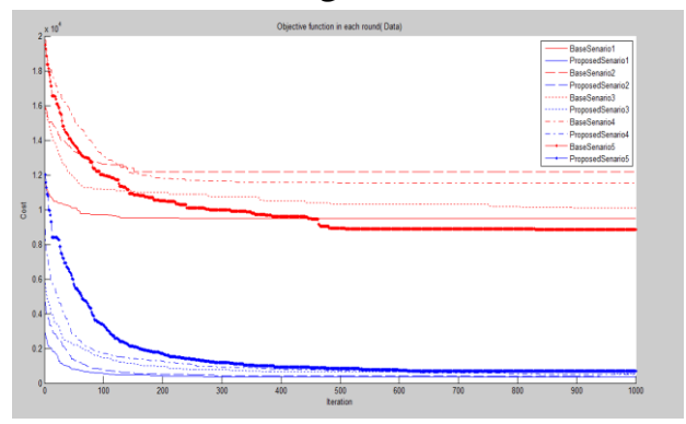
Fig. 4. Objective function
