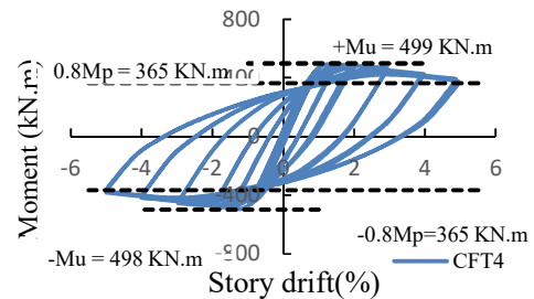
Fig. 21. Connection moment-story drift hysteresis curves D=405 mm - t_f=12.5 mm
