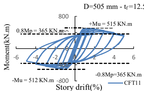
Fig. 23. Connection moment-story drift hysteresis curves D=505 mm - t_f=12.5 mm
