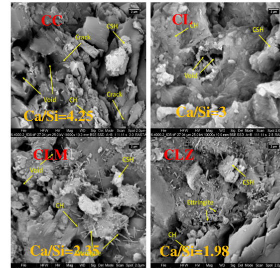
Fig. 6. SEM analysis of different mixtures after water curing condition
