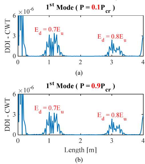
Fig. 10. DDI diagram of the 1 st mode resulting from continuous wavelet analysis of D3 damage state under the effect of axial load (a) 0.1P_{cr} , (b) 0.9P_{cr}
