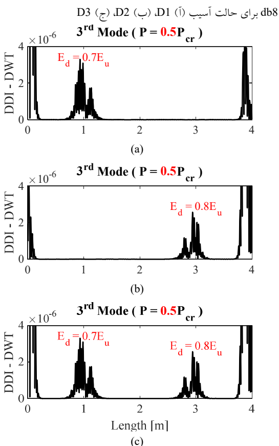
Fig. 9. DDI diagram of the 3 rd mode resulting from discrete wavelet analysis of the db8 function for the (a) D1, (b) D2 and (c) D3 damage state
