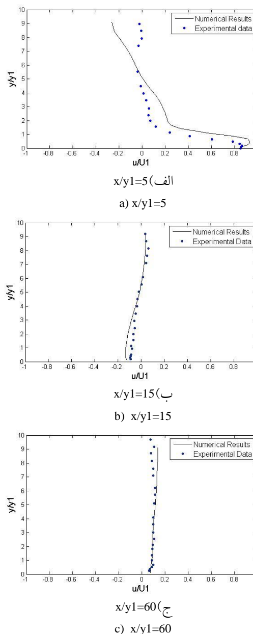
Fig. 5. Dimensionless profile of horizontal component of speed at (z=0) in Model-1
