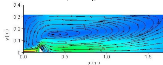
Fig. 7. Flow Pattern and vortex location at (z=0) in Model-1
