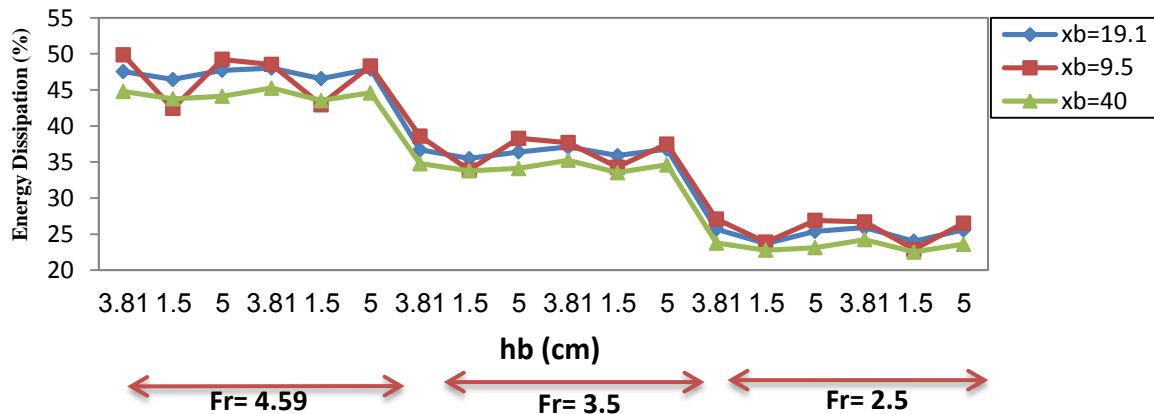
Fig. 10. Effect of block's distance from sluice gate on energy dissipation
