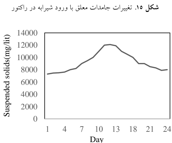
Fig. 15. Changes in suspended solids by the arrival of leachate in the reactor
