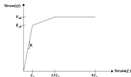
Fig. 2. Mechanical behavior characteristics of bolts
