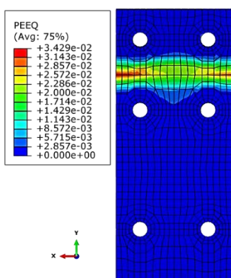
Fig. 8. Plastic Strain of CT1B-6
