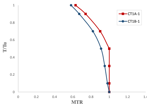
Fig. 15. Torque ratio vs. MTR curve
