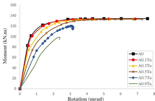
Fig. 16. Moment vs. rotation curve in CT1A-1 in bending and torsion combination
