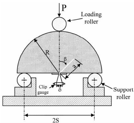
Fig. 5. Schematic of sample loading[4]
