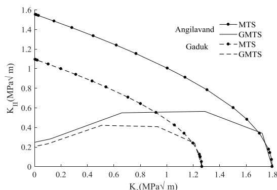
Fig. 17. Fracture curves based on the MTS and GMTS criterion for tested specimens
