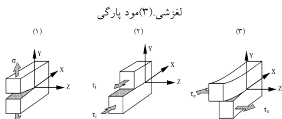
Fig. 1. Three modes. (1) opening mode. (2) shearing mode (3) tearing mode
