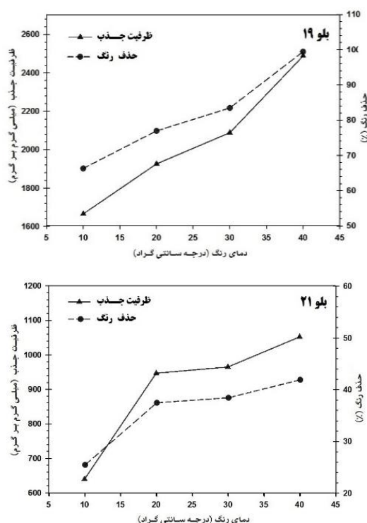
Fig. 10. Diagram the effect of Temperature on the uptake and absorption capacity of reactive dyes Blue 19 and Blue 21
