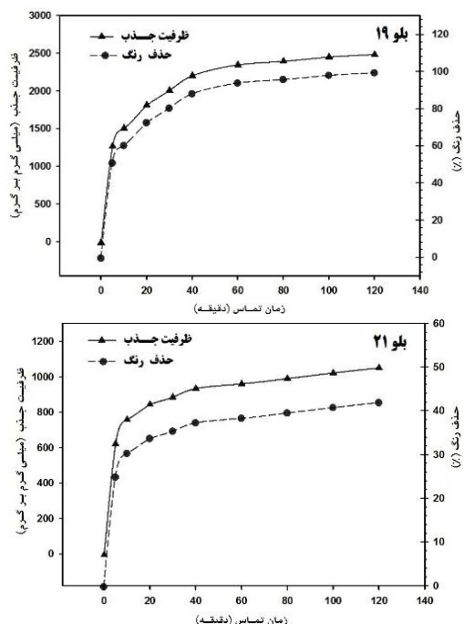
Fig. 11. Diagram the effect of Time on the uptake and absorption capacity of reactive dyes Blue 19 and Blue 21
